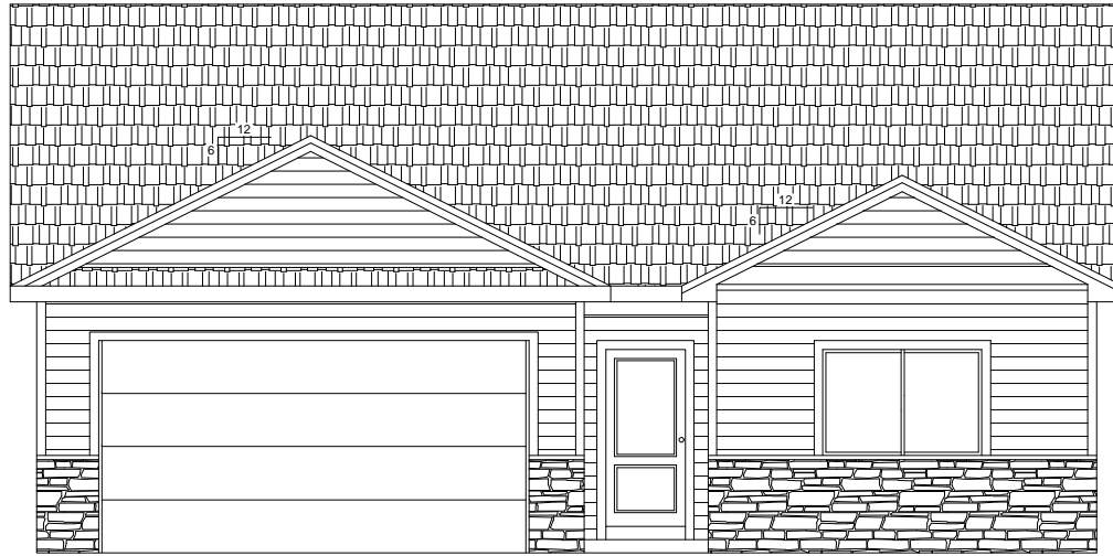
FRONT ELEVATION
